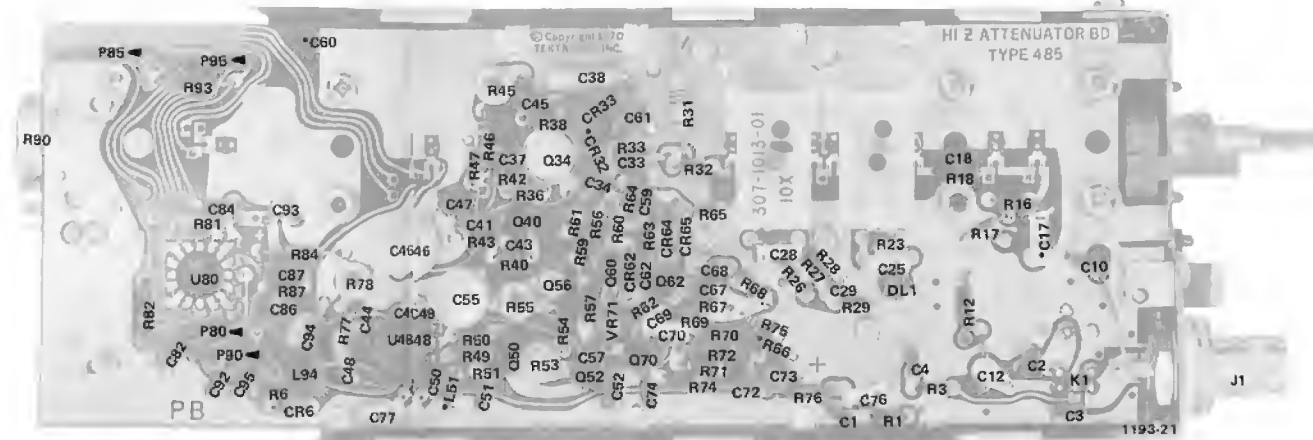
Fig. 8-2B. A3 Hi Z Attenuator board (485 & 485-1 only) SN B010100-B155789.
