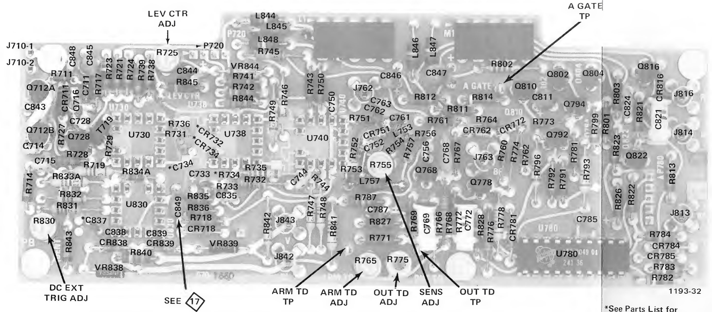
Fig. 8-7A. A8 A Trigger board (485 only).
