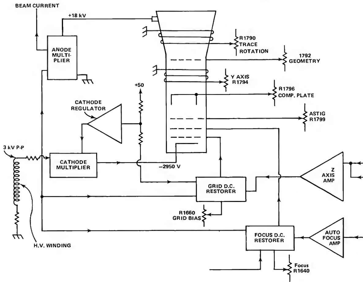
Fig. 3-7. CRT circuit block diagram.
