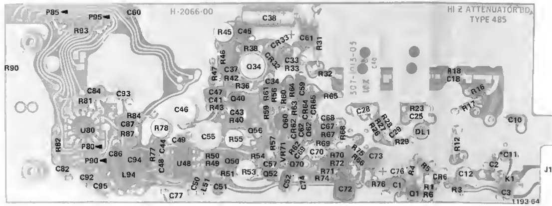
Fig. 8-2A. A3 Hi Z Attenuator board (485 & 485-1 only) SN 8155790-up.
