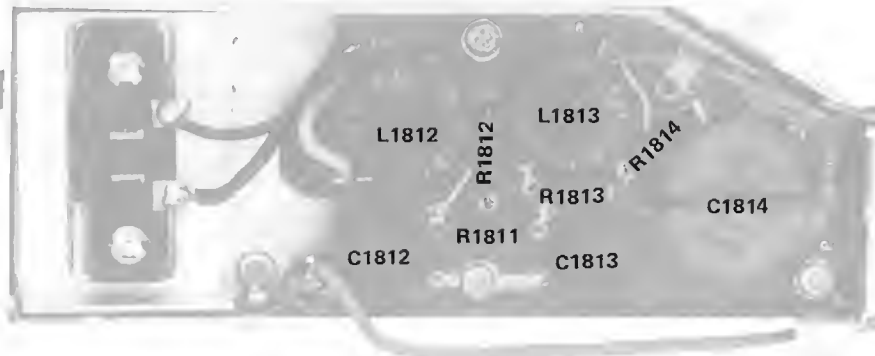
Fig. 8-21. A16 Line Filter board.
